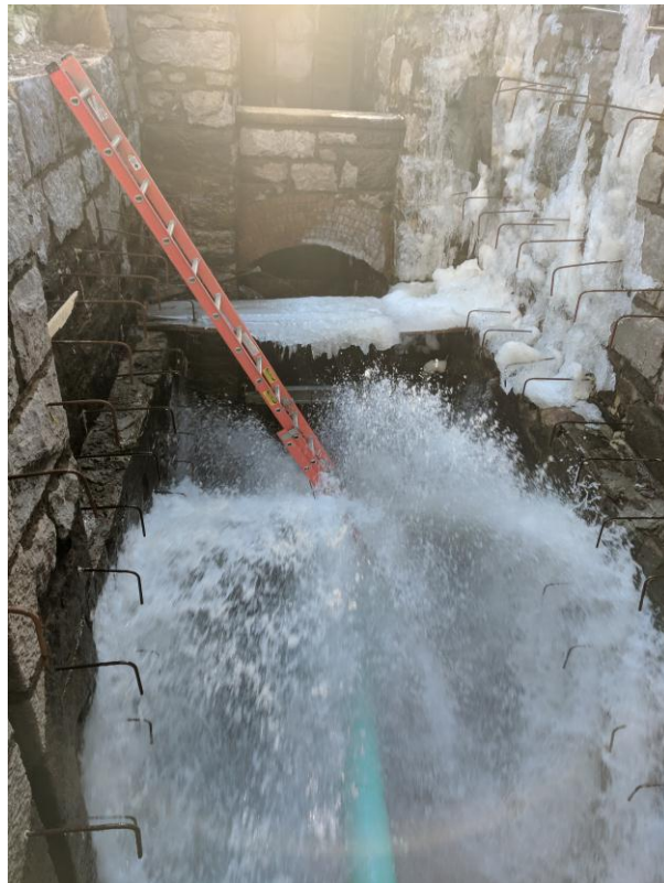
Flow after opening 18" dia. bulkhead penetration.
